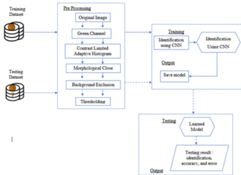
Figure 1: The Workflow of our methodology
