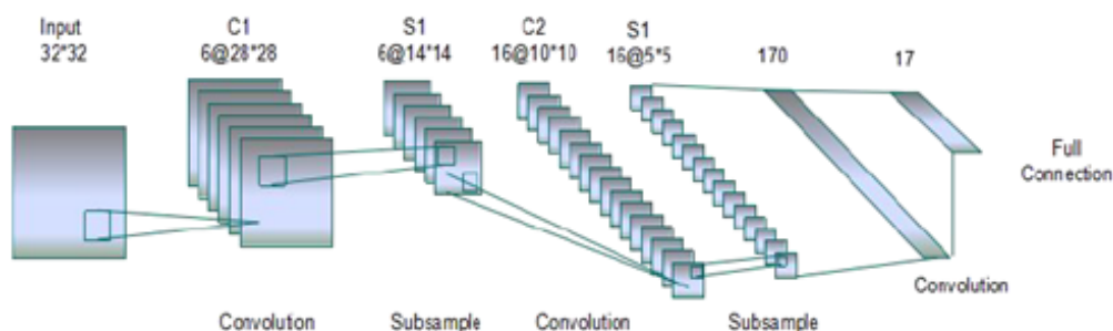
Figure 2: CNN Architecture [8]
